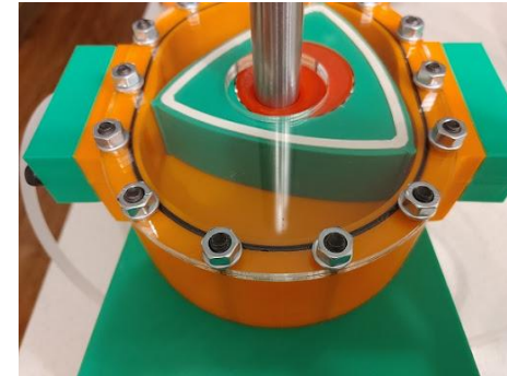
Wankel engine
