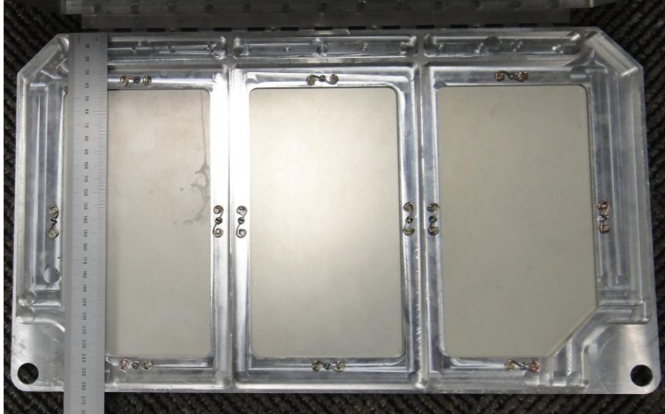
Inside of front door showing the 3 removable panels
